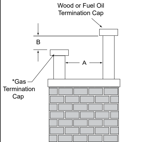
Figure 4.2 Staggered Termination Caps
