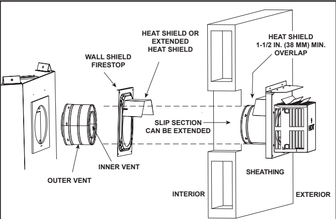
Figure 7.16 Venting Through the Wall
