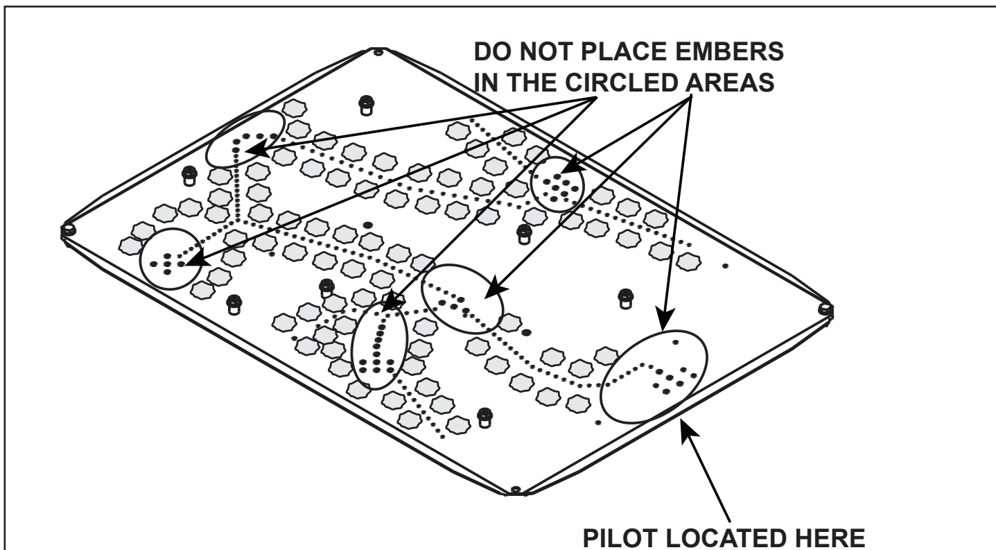
Figure 11.12 Placement of Embers
