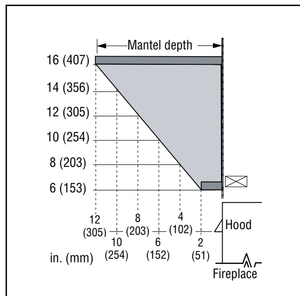
Figure 5A - DRL3500 Series, Standard Installation
