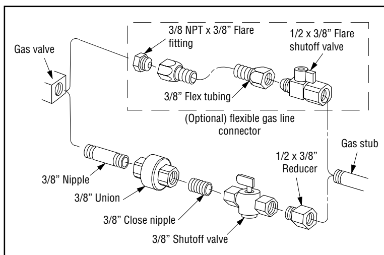
Figure 35 - Gas Line Connection
