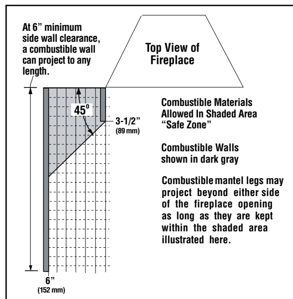
Figure 5C - Combustible Side Clearances
