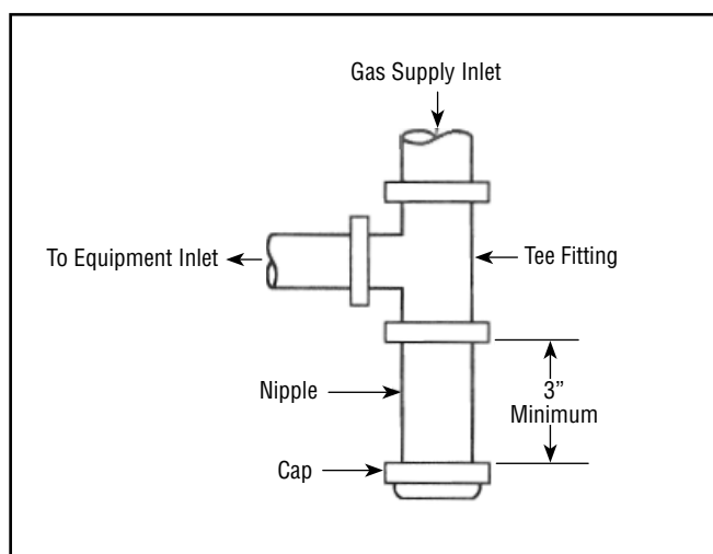
Figure 34 - Sediment Trap
