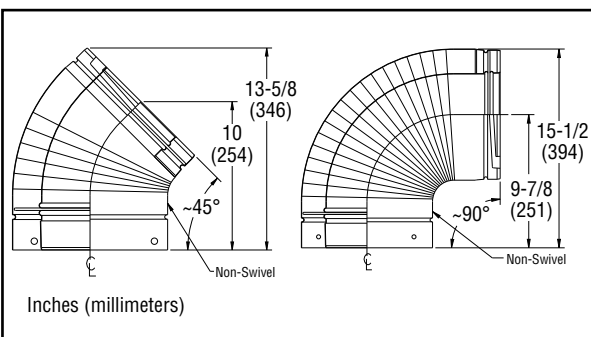
Figure 17 - Elbow Dimensions
