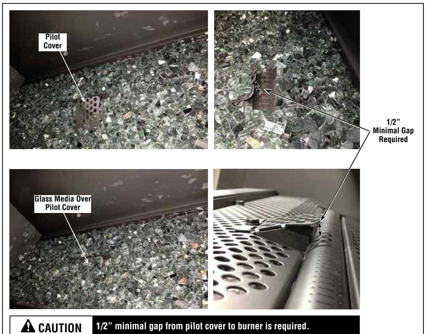
Figure 48 - Removing Sticker and Placing Glass Media Over Pilot Cover.
