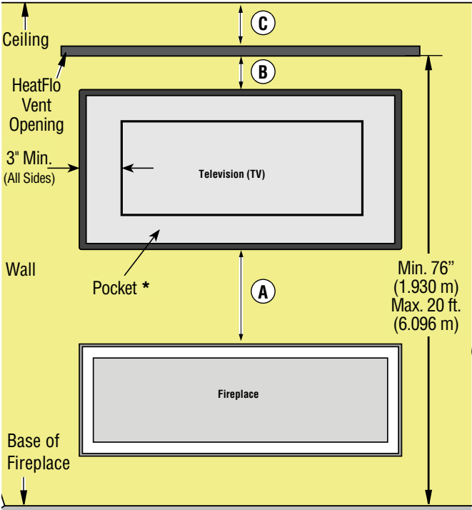
Figure 6A - Dimensions for Television (TV) Installed Above Fireplace on a Recessed Wall Pocket
