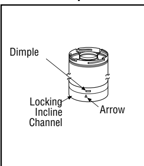
Figure 16 - Connected vent components
